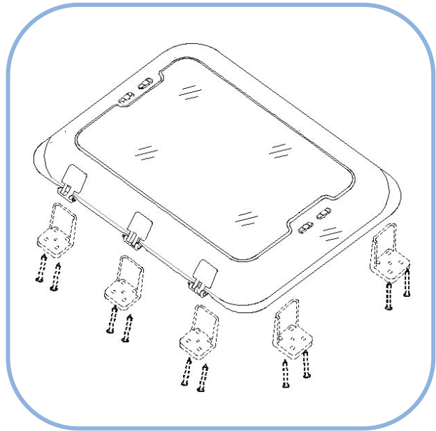
Diagram 5. Screw the outer shell
