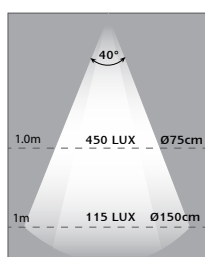
LUX-Distance Curve
