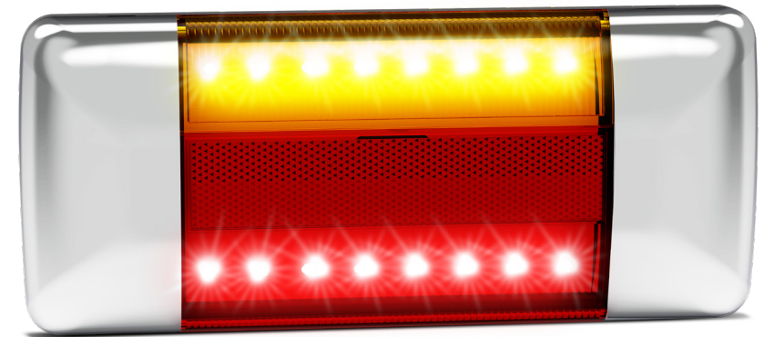
Stop/Tail/Indicator/Reflector 223CARM2 - Twin Blister
