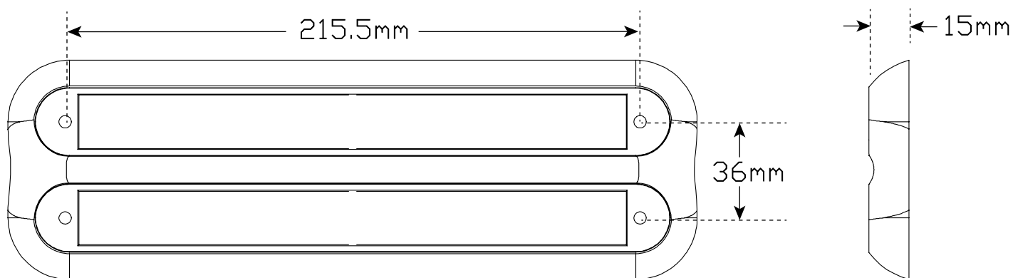
Bracket without lamp installed
